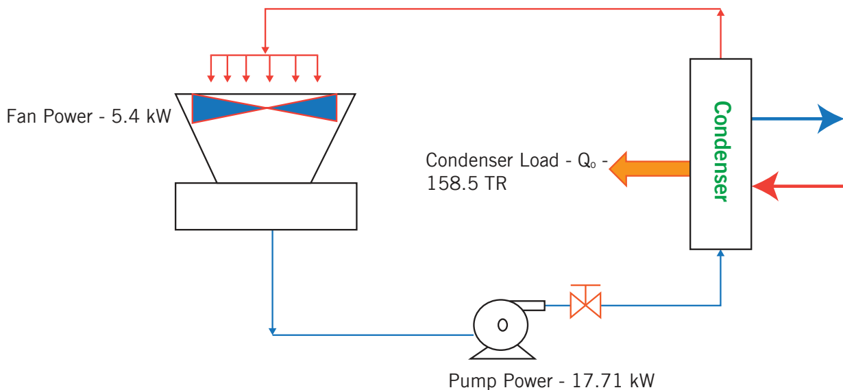
Figure 21: Existing Condenser System
