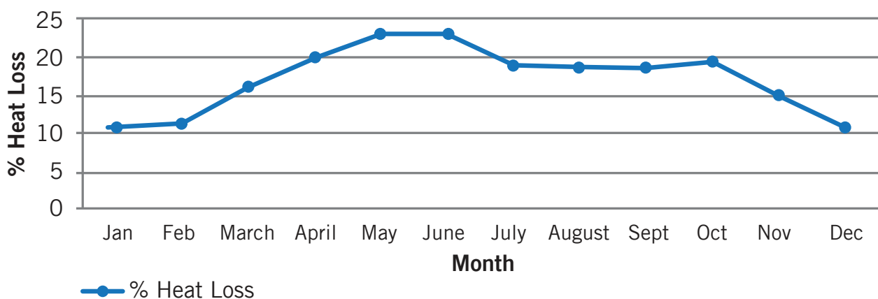
Figure 24: Typical operating efficiency analysis for different seasons
