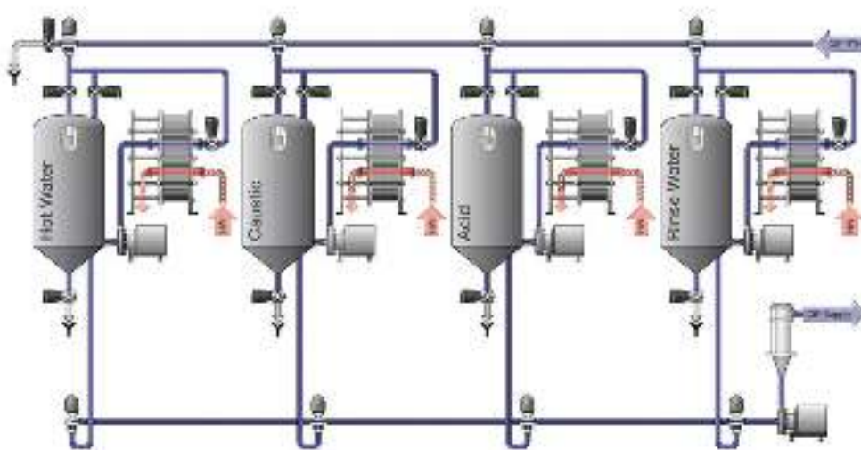
Figure 11: Auto CIP – (Source Alfa Laval)
