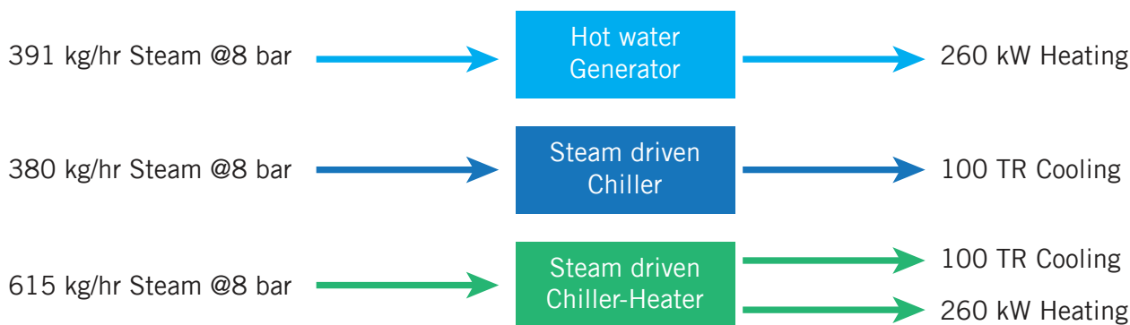
Figure 32: Comparison over conventional system
