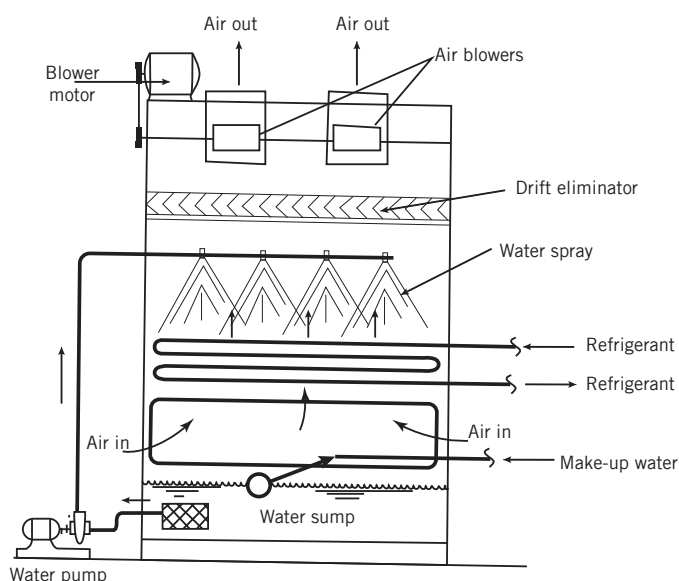
Figure 22: Evaporative Condenser
