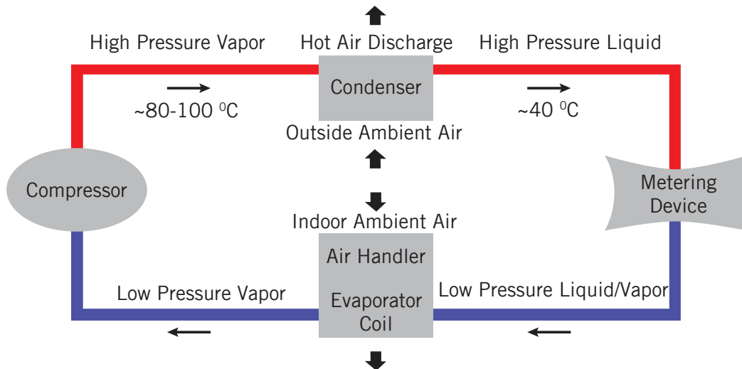
Figure 34: Vapor Compression Cycle
