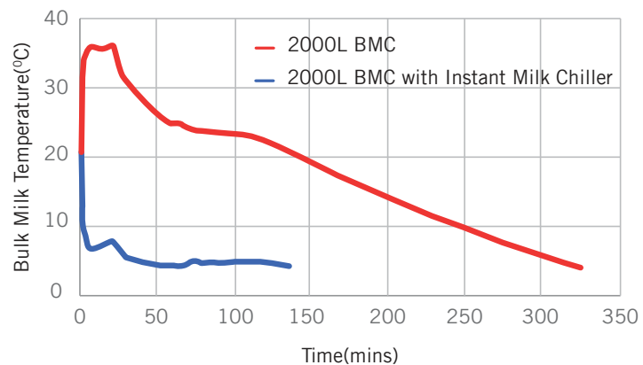
Figure 39: Cooling time with and without instant milk chiller
