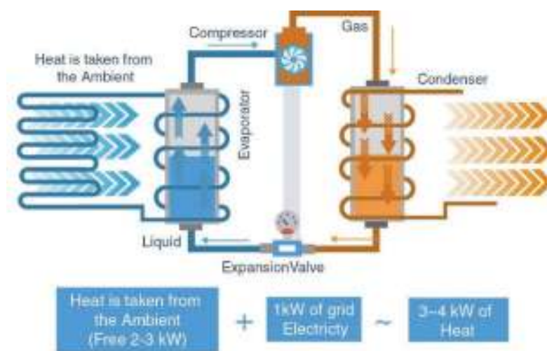
Figure 36: Heat Pump
