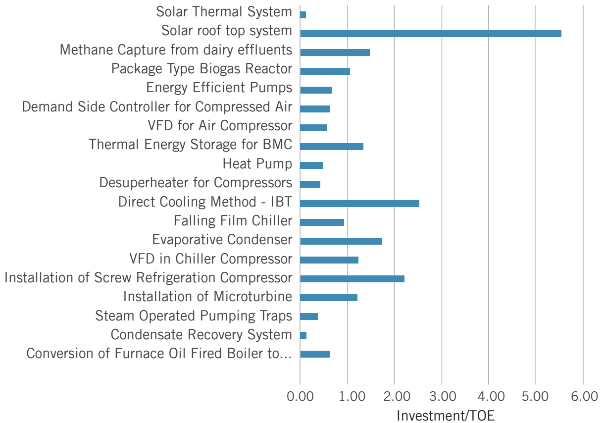
Figure 54: Unit Abatement Cost - Energy Efficient Technologies
