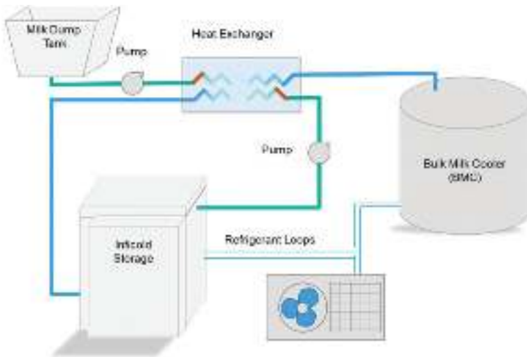
Figure 38: Schematic layout for Instant Milk Cooler
