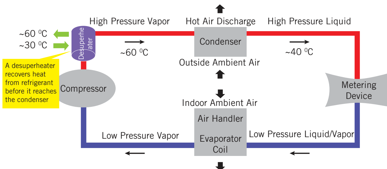
Figure 35: WHR from chiller compressor
