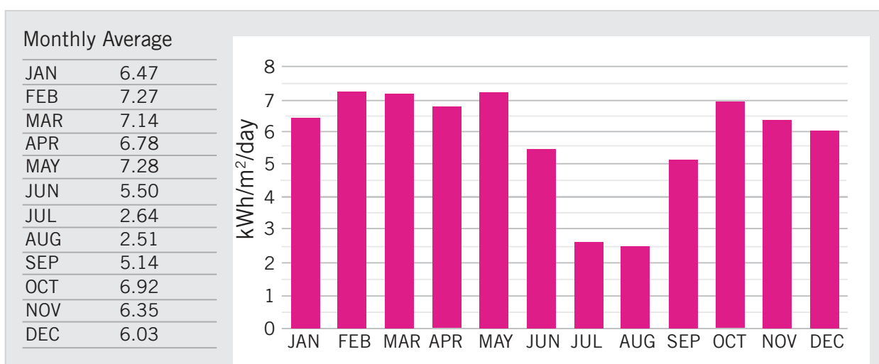
Figure 48: Solar Irradiance
