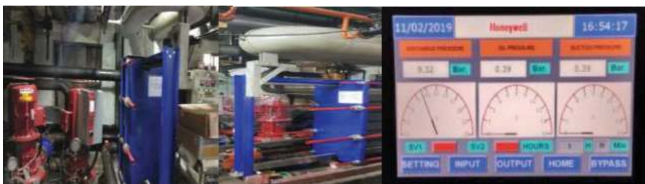
Figure 25: Post Implementation – Direct Cooling Method
