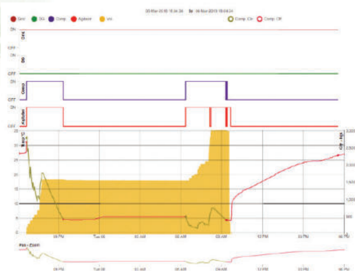
Figure 37: Chilling graph
