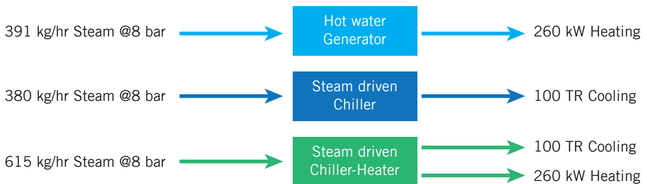
Figure 26: Comparison over conventional system
