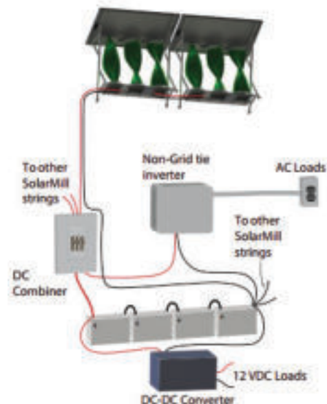
Figure 52: Hybrid mill connected to loads
