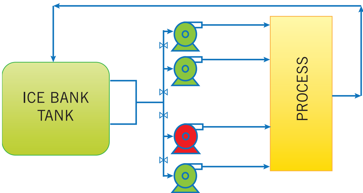
Figure 31: Existing pumping layout
