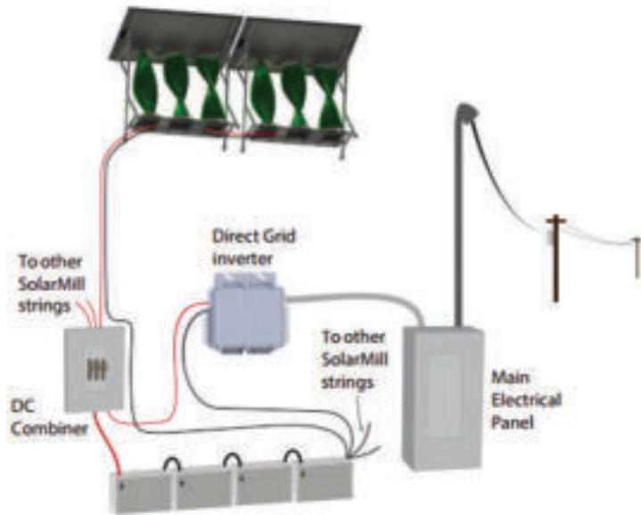
Figure 51: Hybrid mill connected to supply
