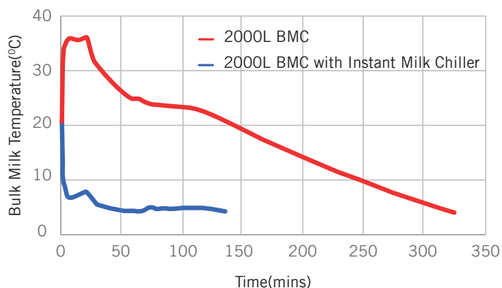
Figure 34: Cooling time with and without instant milk chiller
