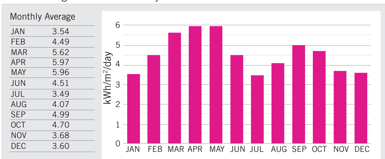
Figure 47: Solar Irradiance
