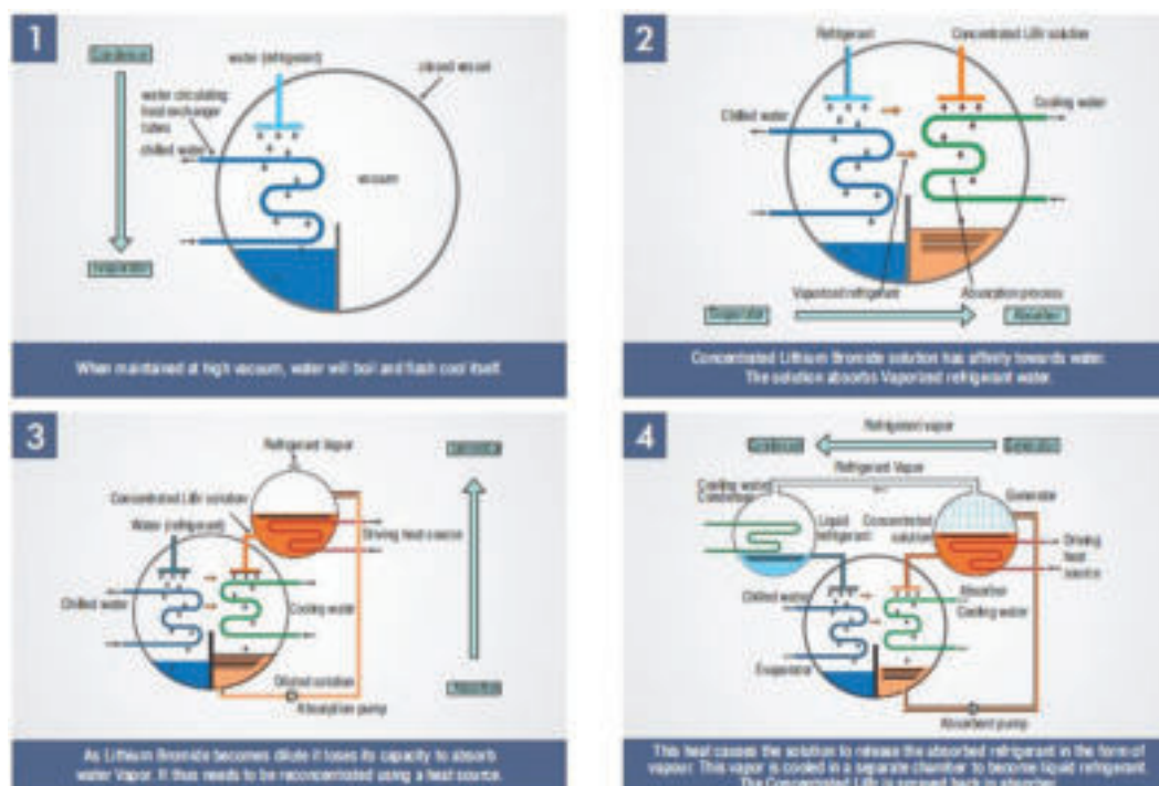
Figure 27: VAM working
