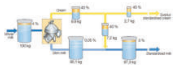
Figure 9: Milk Standardization Process
