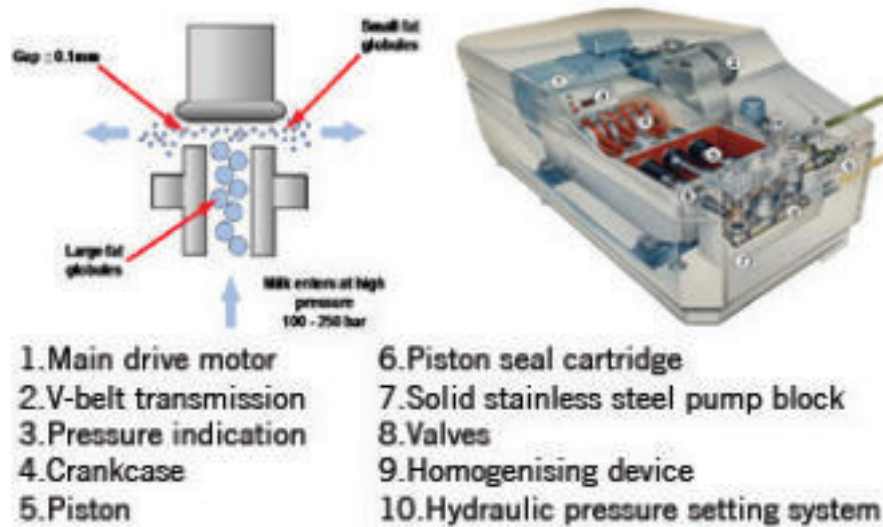
Figure 10: Homogenization Process
