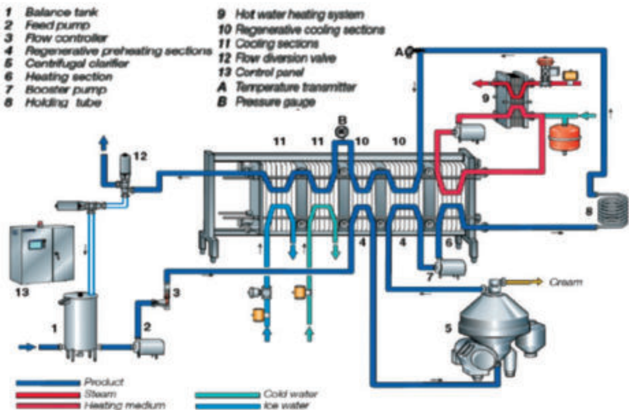
Figure 46: Pasteurization process
