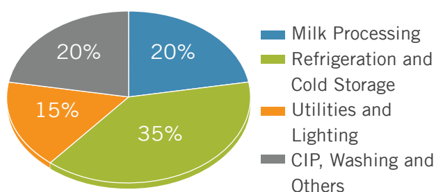
Figure 14: Energy Balance of a Dairy Plant
