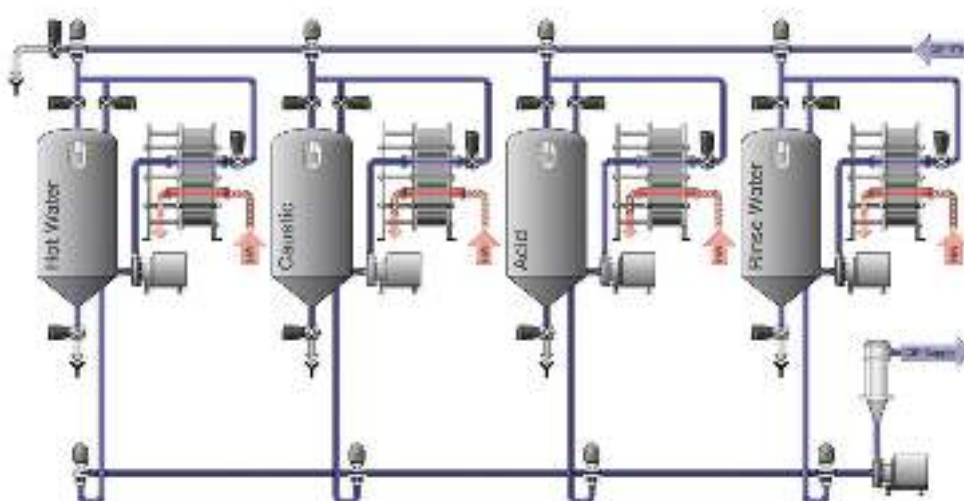
Figure 12: Auto CIP – (Source Alfa Laval)
