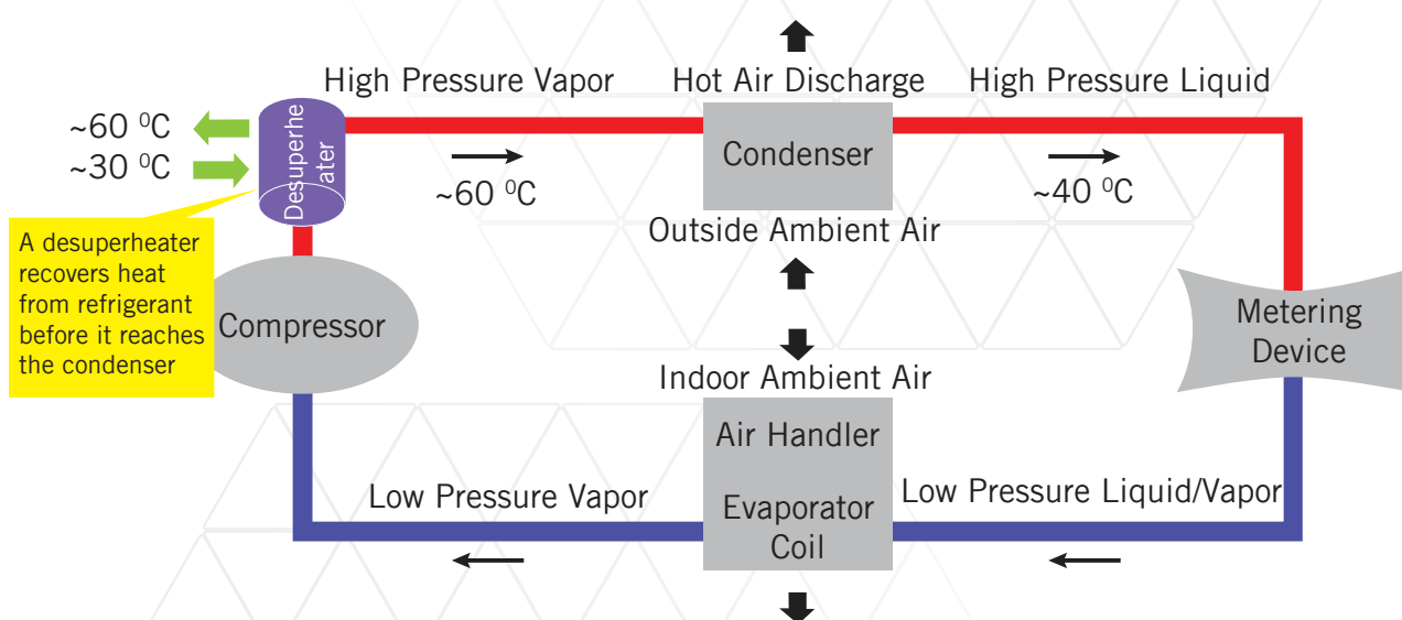
Figure 30: WHR from chiller compressor
