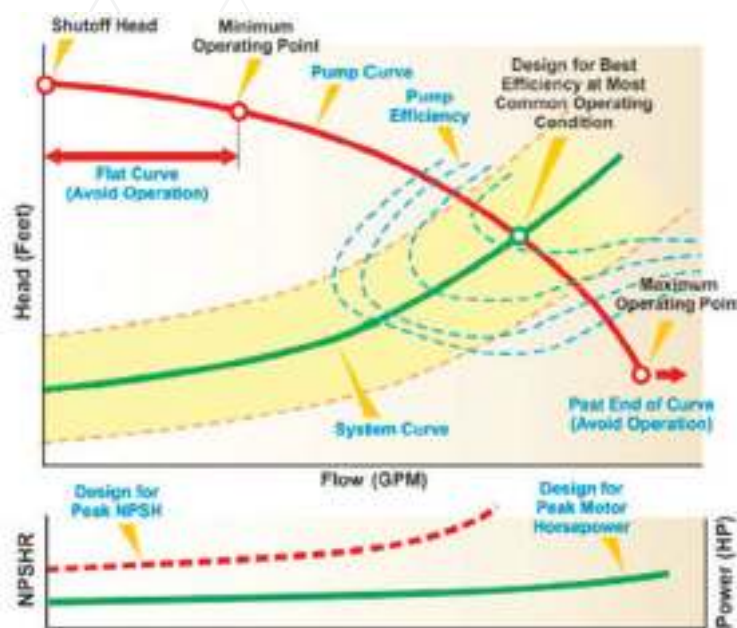
Figure 42: Pump Characteristic Curve
