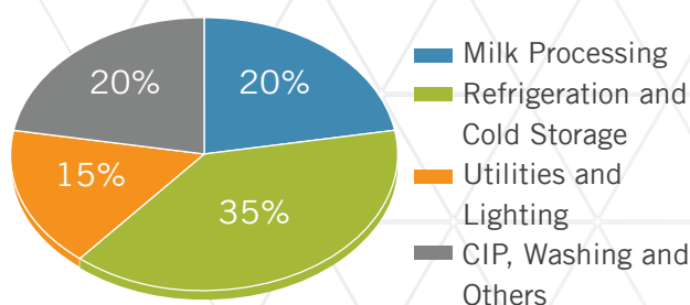
Figure 15: Energy Balance of a Dairy Plant
