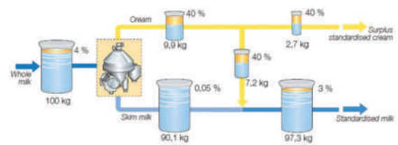
Figure 10: Milk Standardization Process
