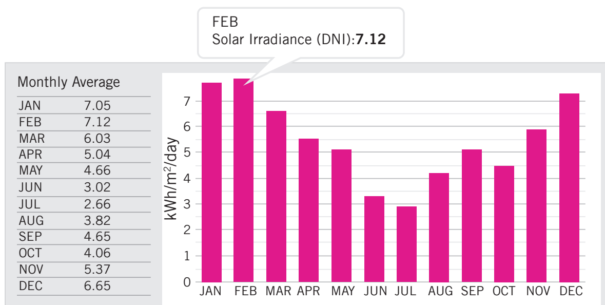
Figure 48: Solar Irradiance
