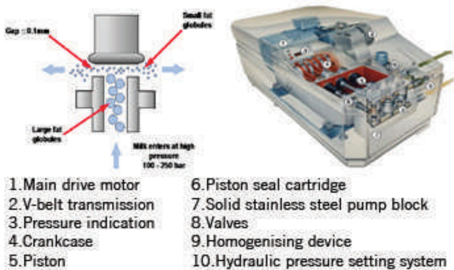
Figure 11: Homogenization Process
