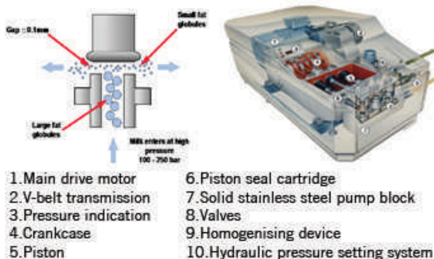
Figure 9: Homogenization Process
