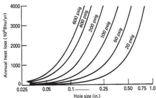
Figure 18: Steam Loss Chart
