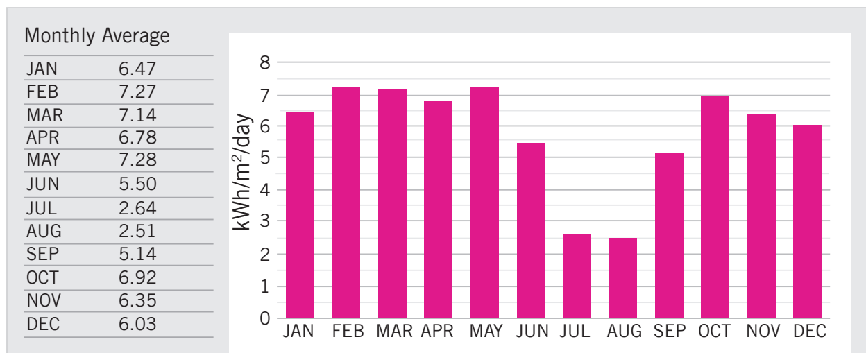
Figure 40: Solar Irradiance
