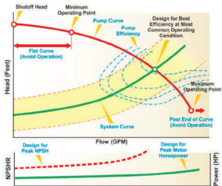
Figure 35: Pump Characteristic Curve
