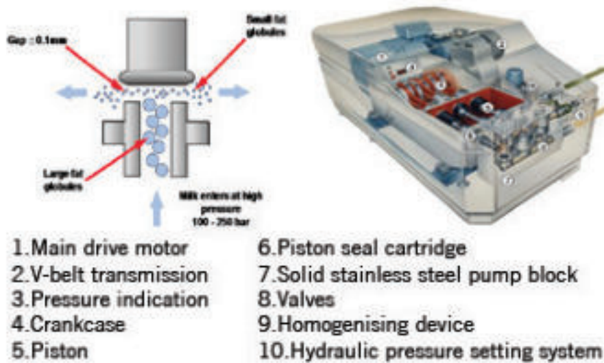
Figure 10: Homogenization Process
