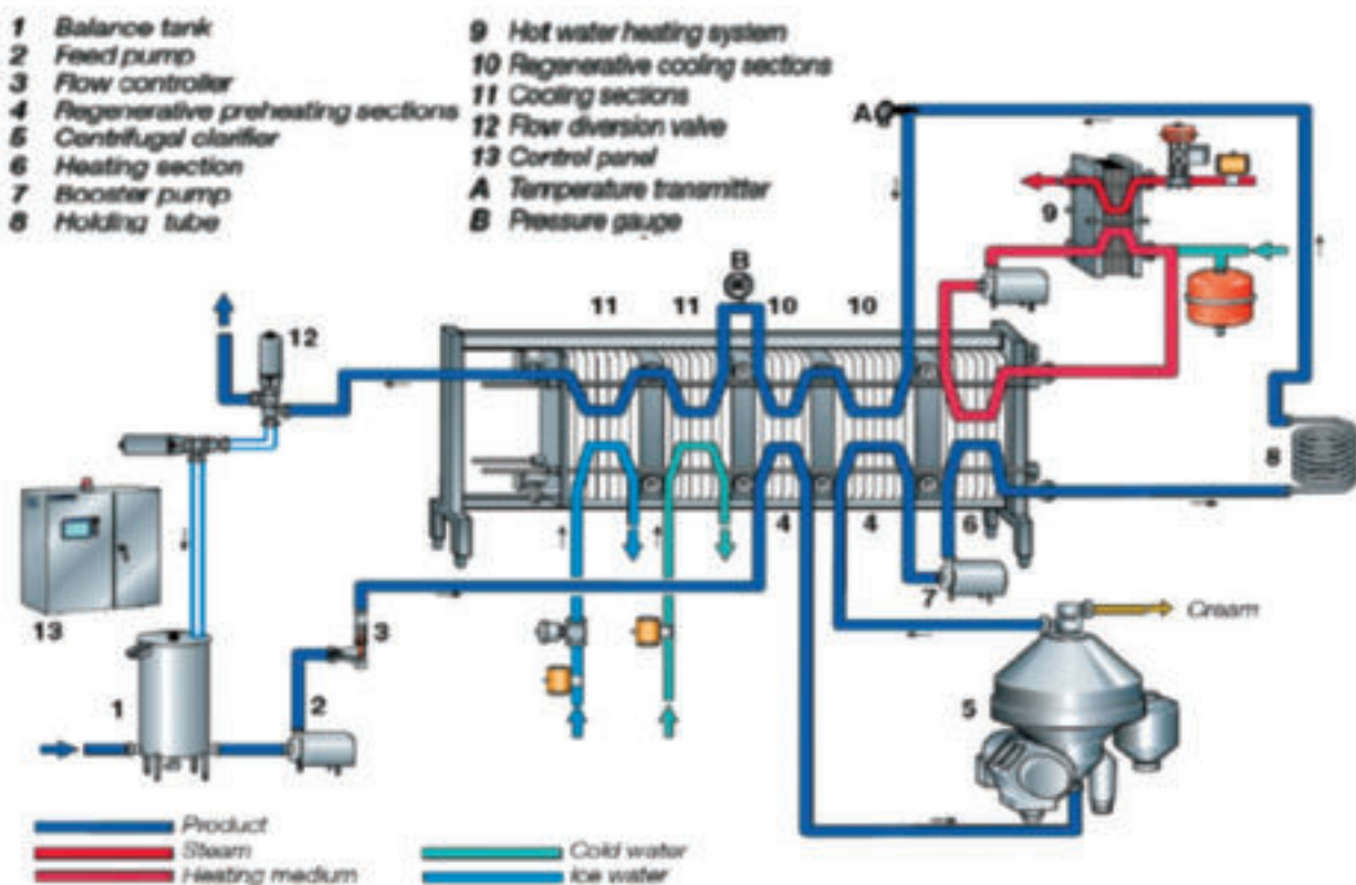
Figure 48: Pasteurization process
