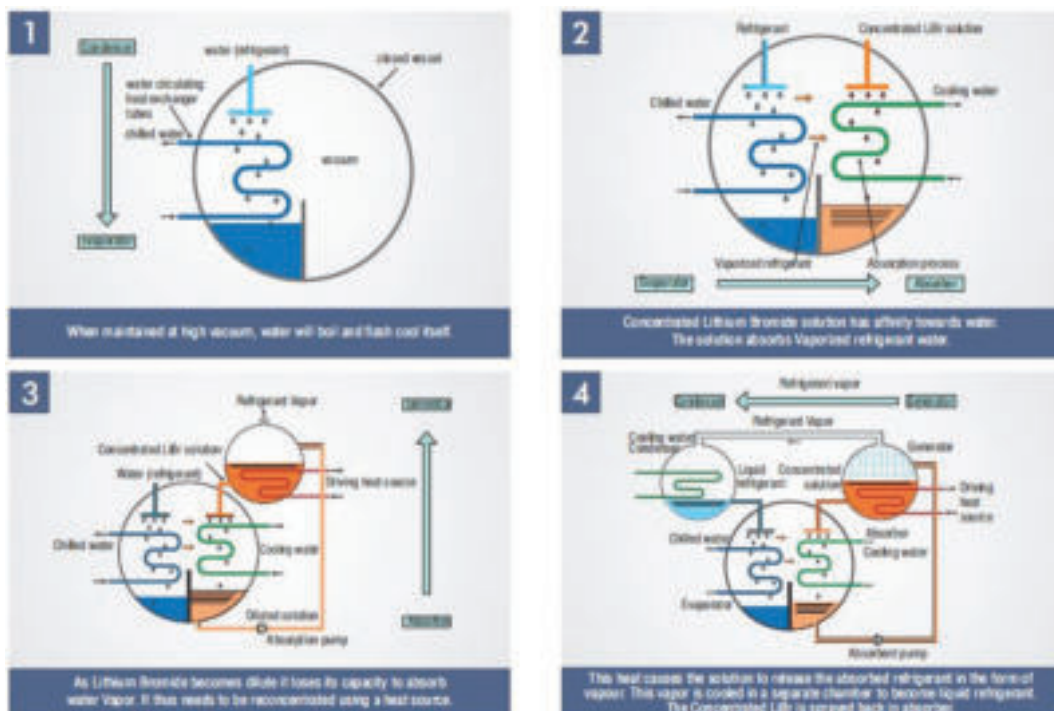
Figure 29: VAM working
