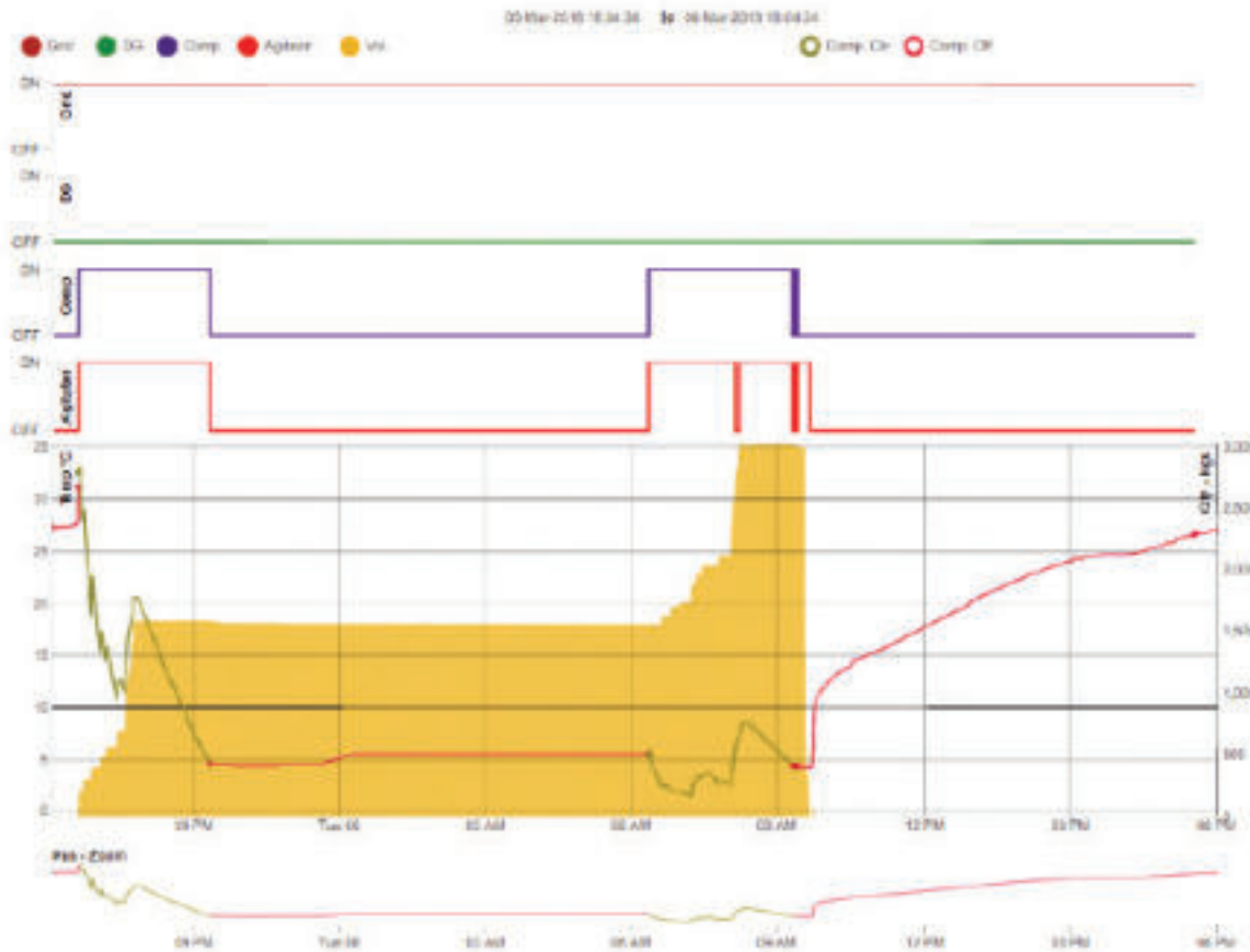
Figure 39: Chilling graph
