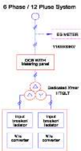
Figure 25: 6 Phase / 12 Pulse System
