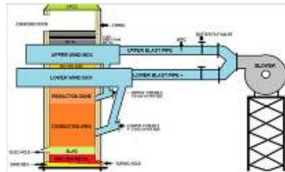
Figure 8: Pictorial representation of divided blast cupola
