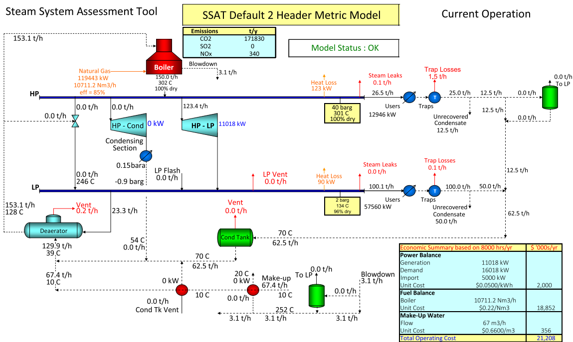
Figure 5b: SSAT “2-Header” Steam System Model
