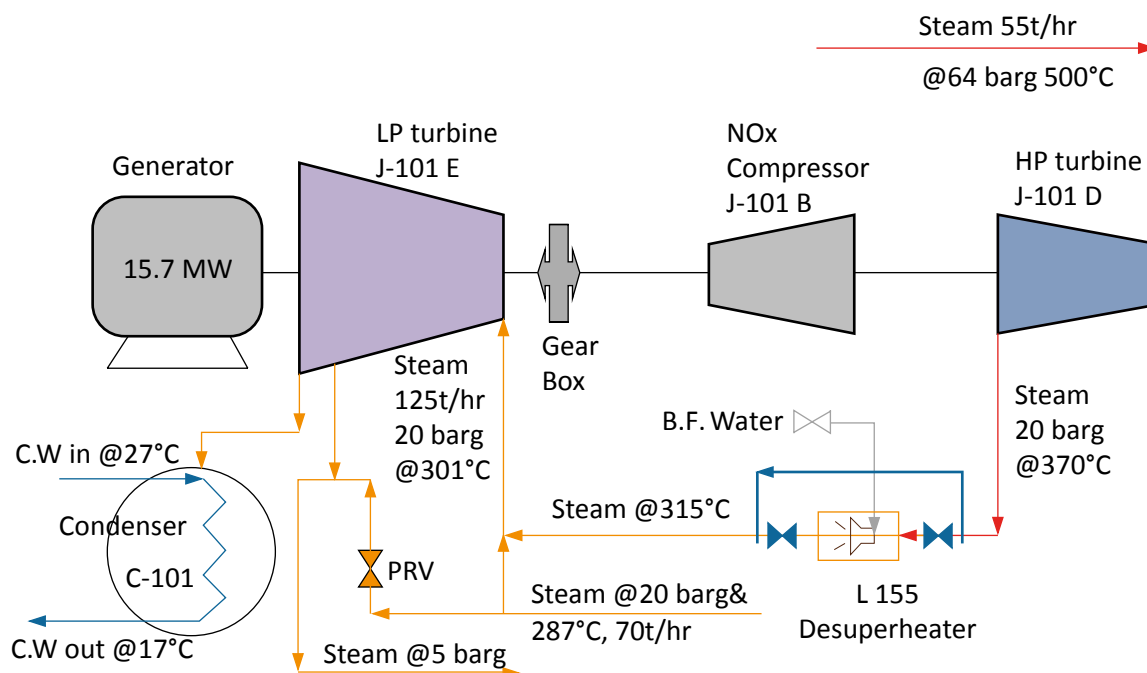
Figure 51: Turbine Operation modified without Desuperheater
