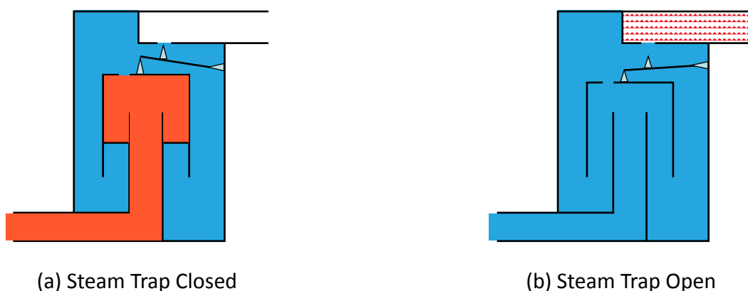
Figure 26: Functioning of Inverted Bucket Mechanical Steam Trap (Courtesy: US DOE Steam BestPractices End User Training)
