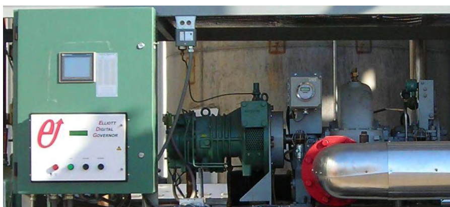
Figure 44: Steam Turbine Driven Screw Chiller
