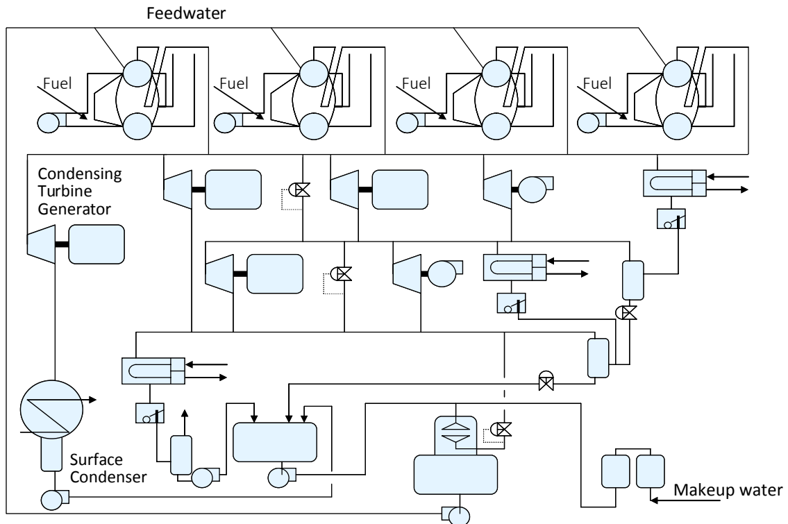
Figure 2d: A 3-Pressure Header w/Condensing Turbine Steam System Line Diagram
